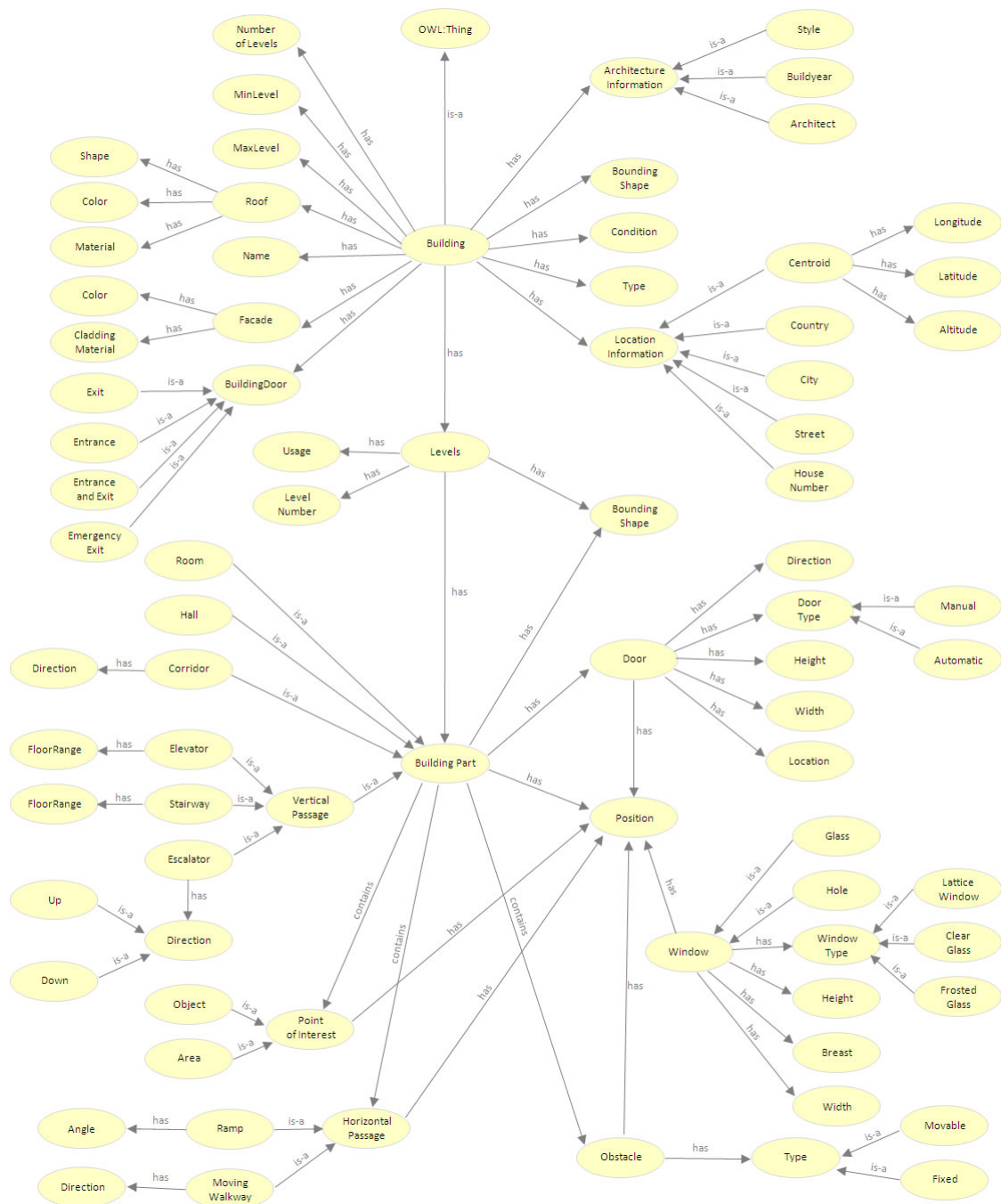
Figure 2. 3D Building Ontology for describing the inside and outside of a building
